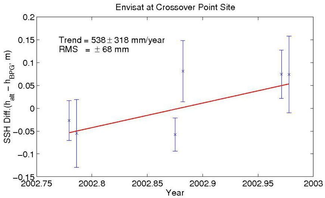
Figure 4.24. Relative comparisons of the ENVISAT ssh with the sea level inferred from the Sabine BPG.
