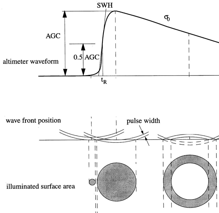
Figure 4.6. The ideal average altimeter waveform for the water and its illumination pattern (Kruizinga, 1997).
