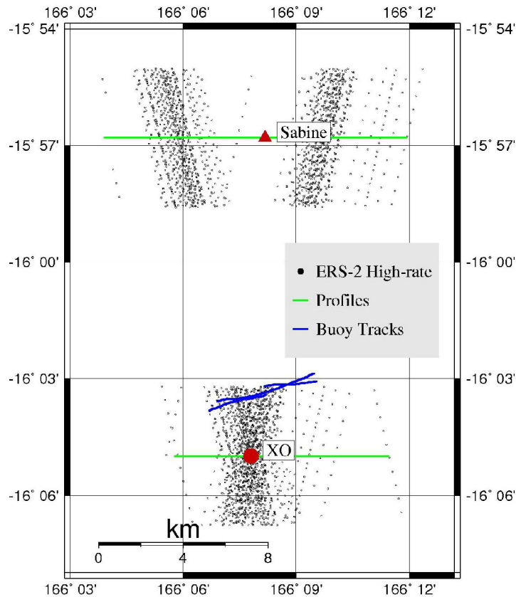
Figure 4.20. The high rate ERS-2 footprints near the Sabine BPG. The buoy tracks were from the 2004 campaign. The nominal parallels are at the Sabine BPG (at 15°56'48" S) and at the crossover (XO) point (at 16°04'59" S).
