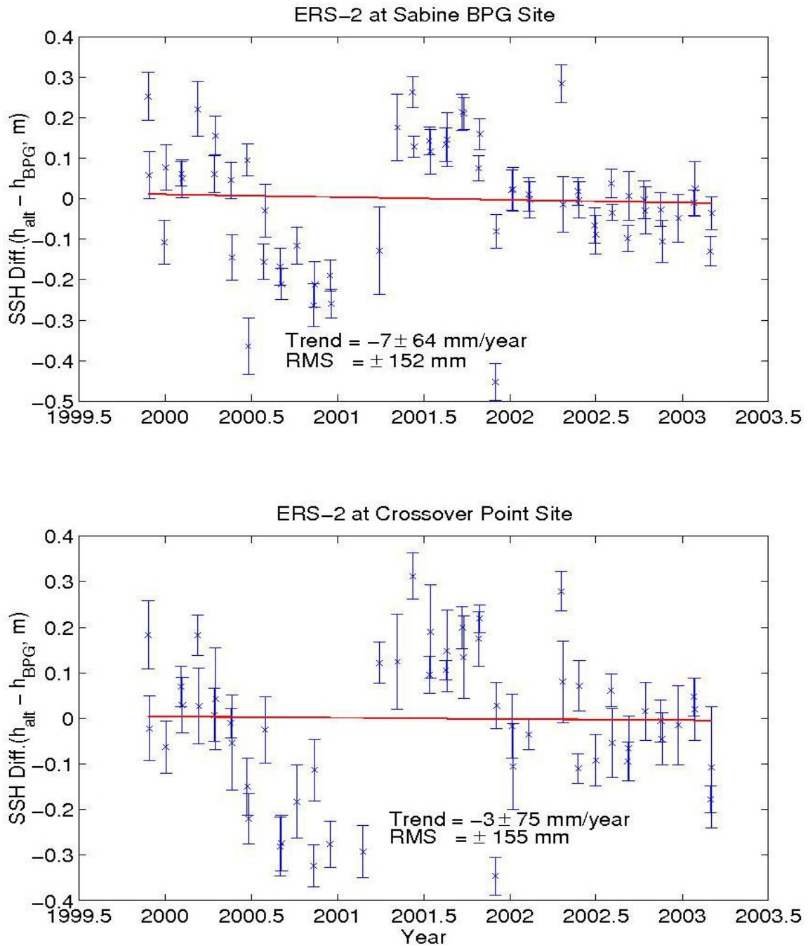
Figure 4.23. Relative comparisons of the ERS-2 ssh with the sea level inferred from the Sabine BPG.
