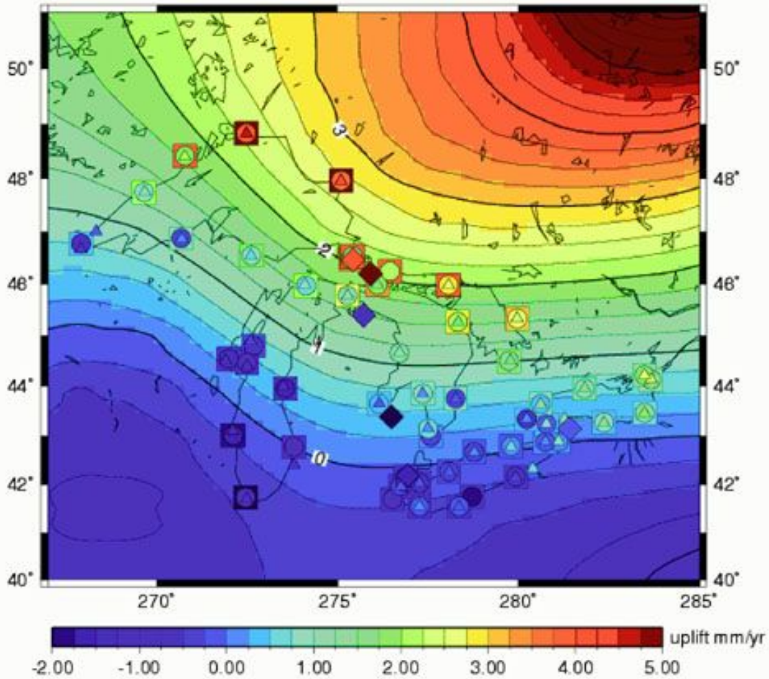
Figure 3.6. Vertical motion based on 50 tide gauges and TOPEX cycles 3–330 in the Great Lakes. Background shows predicted vertical motion of the ICE-4G VM2 model (Peltier, 2002). Triangles represent estimates of a tide gauge only analysis by Mainville and Craymer (2003). Squares indicate GIA model predictions of Mitrovica (Lithospheric thickness = 120 km, Upper mantle viscosity = 1 \times 10^{21} Pas, lower mantle viscosity = 3 \times 10^{21} Pas). Diamonds are USGS GPS velocity estimates (Figure adapted from Kuo et al., 2004a).
